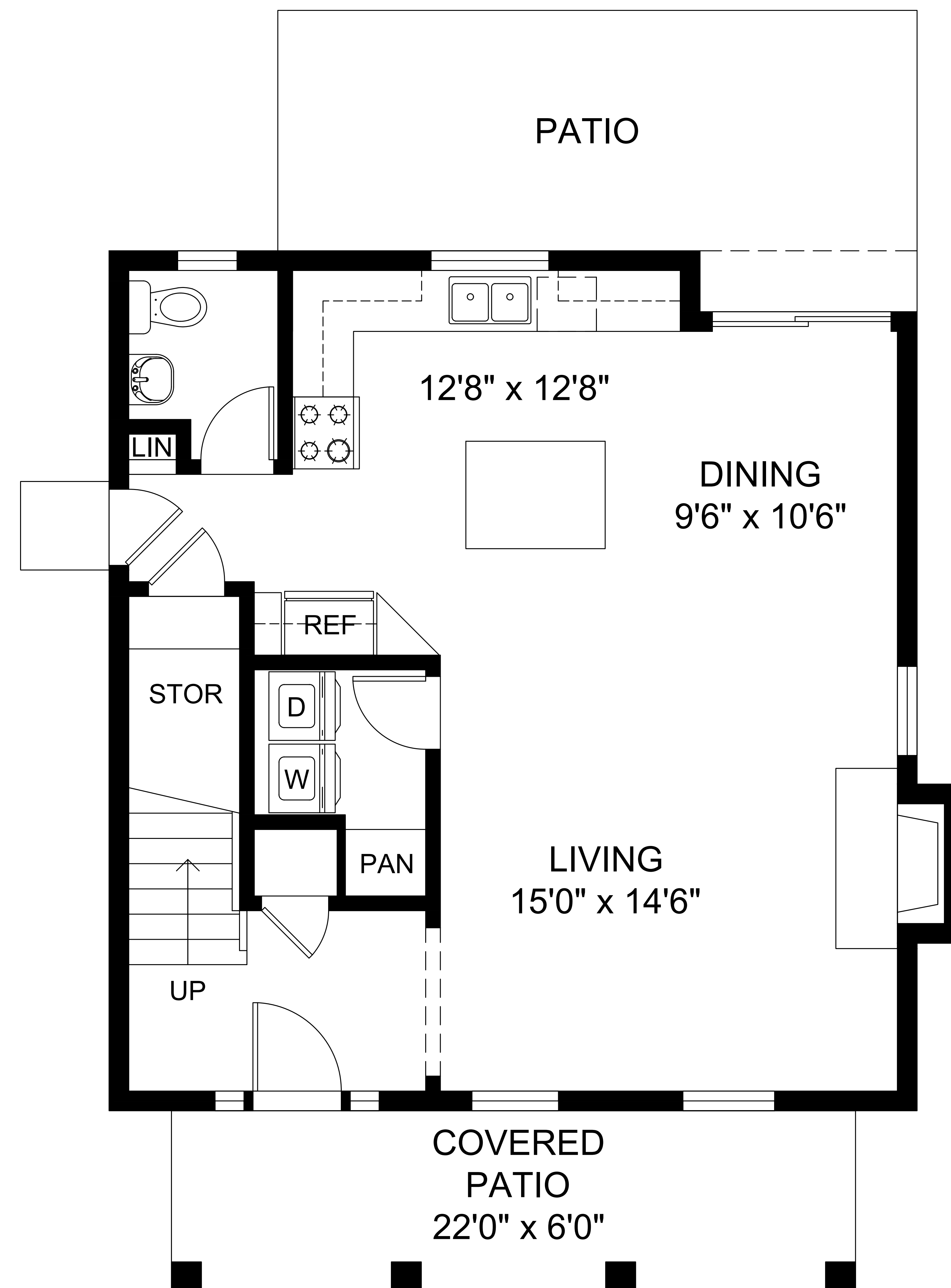
FIRST FLOOR
